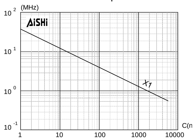
Resonant VS Capacitance
