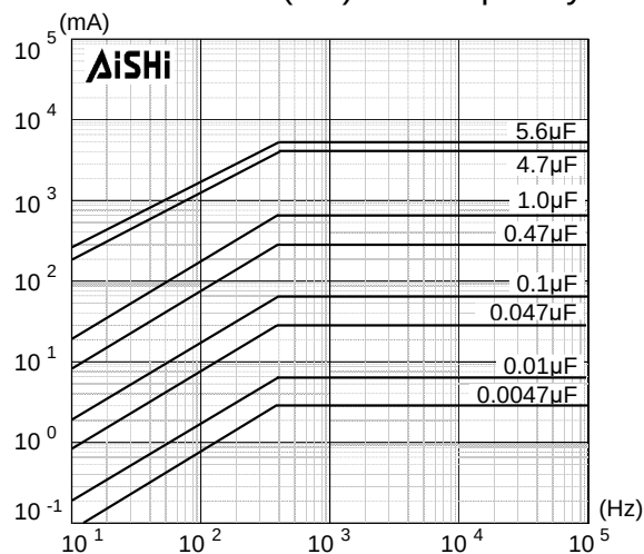
Maximum Current ( I_{rms} ) Vs Frequency
