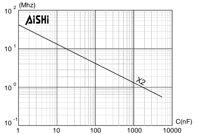
Resonant VS Capacitance
